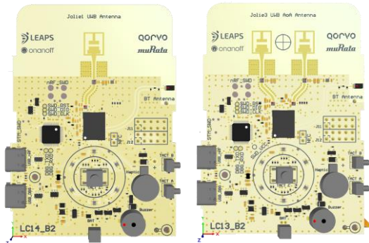
Figure 4: Top view of the board (Left - LC14, Right - LC13)
